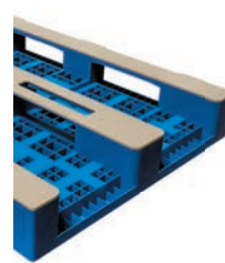
PALLET RE-INFORCED (suitable for use in warehouse racks)
